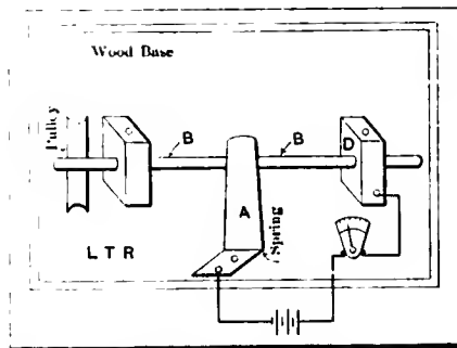
Fig. 2—Apparatus devised to test the presence of oil film between shaft and bearings
